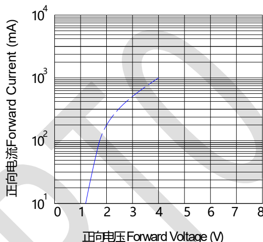
电流vs电压曲线图 Current & Voltage Curve
